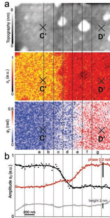
Fig. 1: s-SNOM image at 0.6 THz of n/p transition in Si; a, simultaneously recorded topography, THz amplitude s_3 , and THz phase \varphi_3 (acquisition time 2.5 min); b, line profiles of height (grey), amplitude (black), and phase (red), obtained by averaging, show that electron density reduces from 2 \cdot 10^{17} \text{ cm}^{-3} in section a along b and c to ca. 3 \cdot 10^{16} \text{ cm}^{-3} , while hole density emerges along d and e to attain a value of 2 \cdot 10^{16} \text{ cm}^{-3} .
