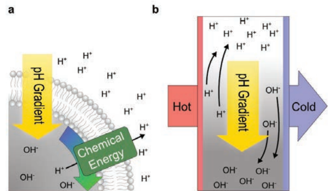
Fig. 1: Formation of pH gradients by chemical or thermal energy. A) Modern cells run on an elaborate protein system to maintain proton gradients across a membrane. Chemical energy is used to pump protons against their concentration gradient which is then harnessed by chemiosmosis. B) Heat fluxes across confined solutions, a common geological setting, induce a movement of ions that results in a stable pH gradient of up to 2 pH units. The charge selective thermophoretic accumulation of buffer molecules such as amino acids, phosphates, or nucleotides keeps the water self-ionization persistently out of equilibrium. The formation of a pH gradient is achieved in a closed system and biomolecules are repetitively exposed to differences in pH.
