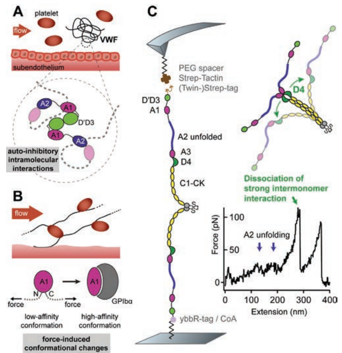
Fig. 1: Large VWF multimers freely circulate in the blood stream in an inactive conformation (A). Upon elevated shear forces occurring at sites of injury VWF is activated both by removal of auto-inhibitory intramolecular interactions and by local conformational changes, resulting in increased platelet binding (B) via the A1 domain. (C) By AFM force spectroscopy, force-induced conformational changes can be studied at the single-molecule level to gain insights into the relation between force, structure and function.
