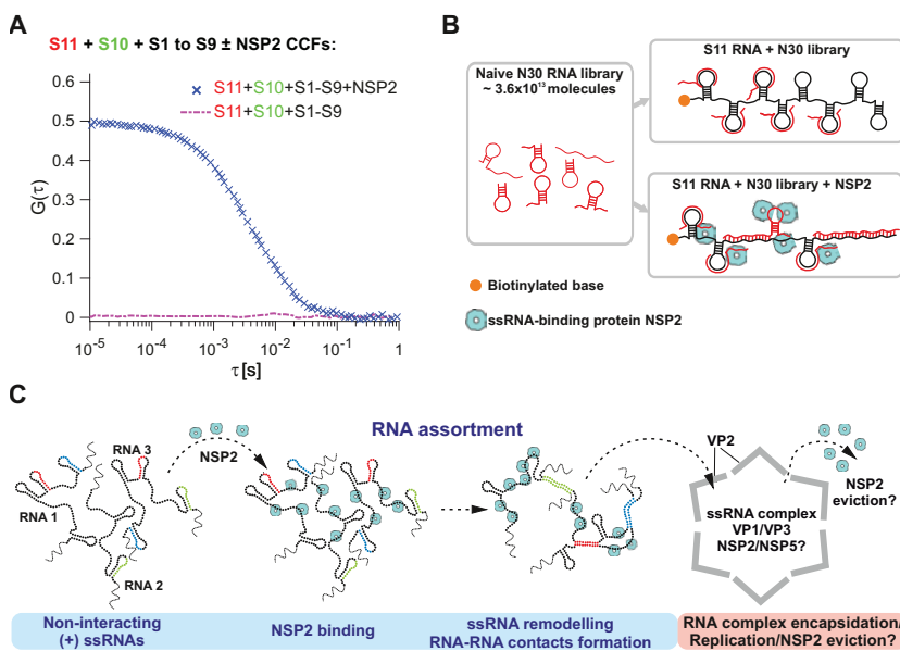
Fig. 1: The Role of NSP2 in Rotavirus Assembly. A) FCCS measurements with fluorescently labeled segments S10 and S11 (in the presence of unlabeled segments S1 and S9) from rotavirus showing a significant increase in cross-correlation signal upon addition of the non-structural protein, NSP2. B) A schematic of SELEX measurements showing the binding of 30 bp RNAs to single-stranded regions of segment S11 in the absence and presence of NSP2. Thereby, we can detect NSP2 induced structural rearrangements of the segment 11 RNA. C) A model of rotavirus RNA assembly where binding of NSP2 rearranges the viral RNA such that it can package a single copy of each RNA.
